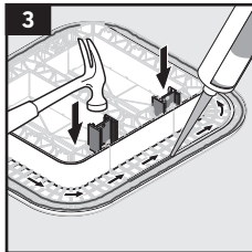
3 Fasten the clips and add sealant.
