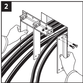
Assemble the frame around the cables.
