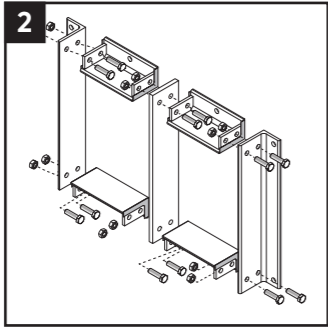
Arrange the frame parts.
