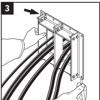
Mark the location of the fasteners using the frame.
