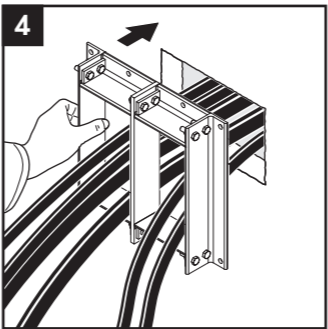
Place the frame against the structure.
