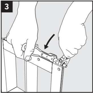
Tighten the fasteners firmly.
