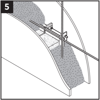
B frame cast in wall.
