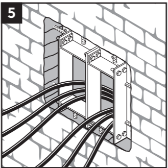
B frame attached to rebar in wall.
