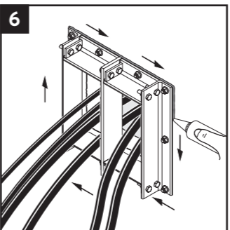
Apply a final string of sealant around the perimeter of the flange.
