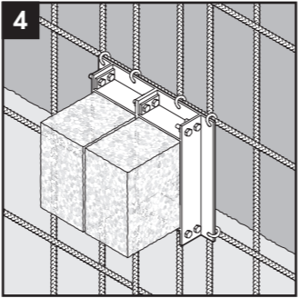
B frame attached to rebar with mold inserts.
