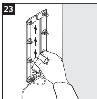
23 Lubricate the sealing surfaces of the frame, especially in the corners. Lubricate the area that will be in contact with the braid sparsely.
