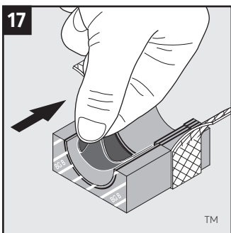
17 Adapt the layers that are in contact with the cable jacket.
