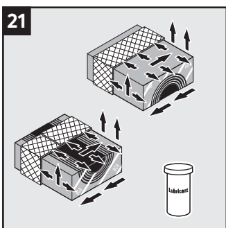
21 Lubricate the sealing surfaces of the spare modules. Do not remove the core.
