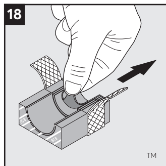
18 Adapt the layers that are in contact with the cable armor.
