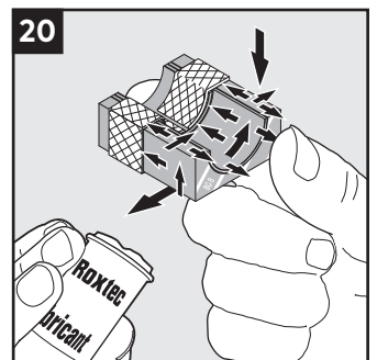
20 Lubricate the sealing surfaces of all modules. Avoid excess lubricant on the braid.
