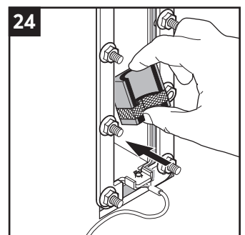
24 Insert the modules at an angle from the backside of the transit according to your packing plan.
