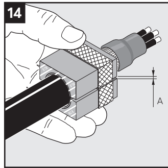
14 Achieve a gap of 0.1-1.0 mm (A) between the module halves by peeling off layers.
