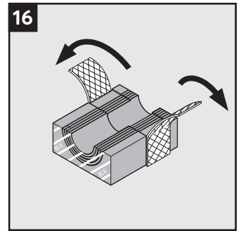
16 Remove the core and fold out the braid. Also see section for modules with multiple openings.
