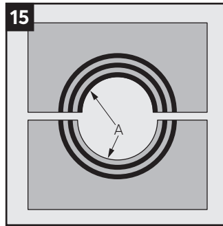
15 The number of layers may not differ (A) by more than one between the corresponding module halves.
