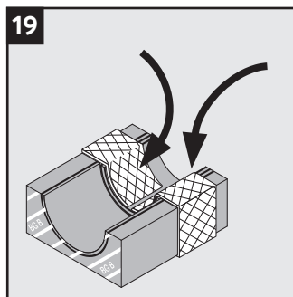
19 Fold the braid tightly inside the module half. Check the gap.
