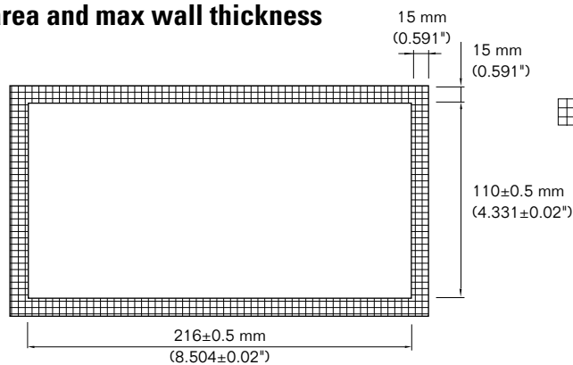
Fig. 7: CF 32 EMC aperture dimensions
