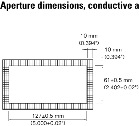
Fig. 6: CF 8 EMC aperture dimensions
