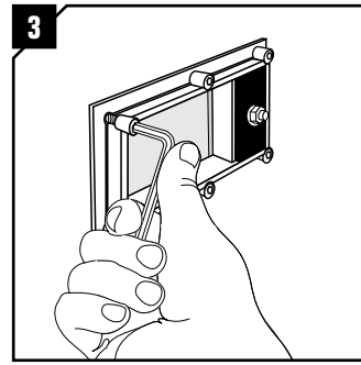
Fasten the hexagon nuts on the backside.
