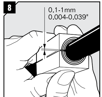
Try to achieve a 0.1–1 mm gap between the two halves when held against the cable/pipe. Use the Ex Gap Gauge.
