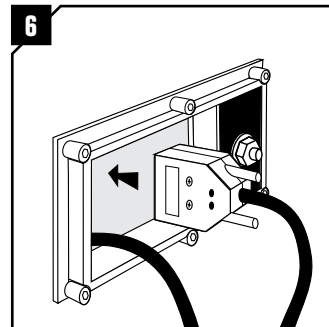
Insert the cables through the frame.
