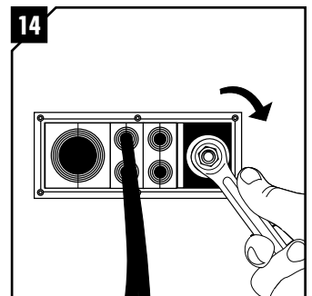
Tighten the compression unit. Minimum 8 Nm.
