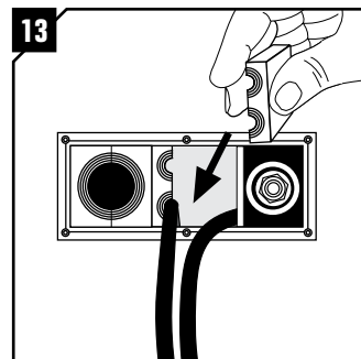
Insert the modules from the inside of the cabinet.
