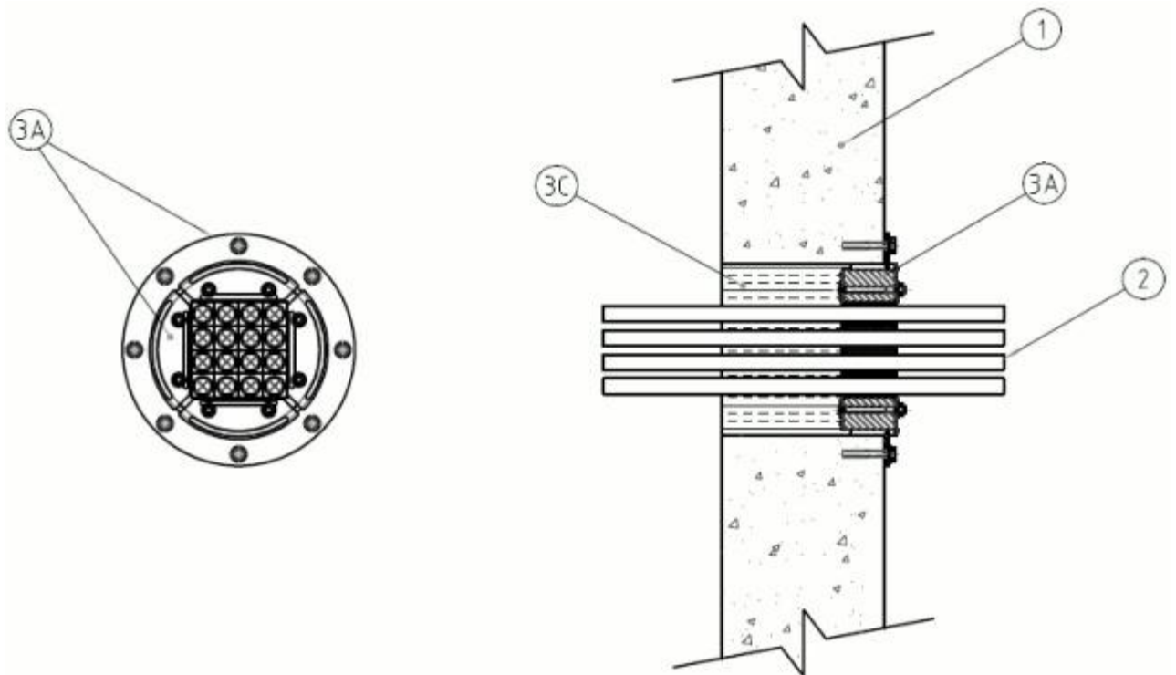
CONFIGURATION B
