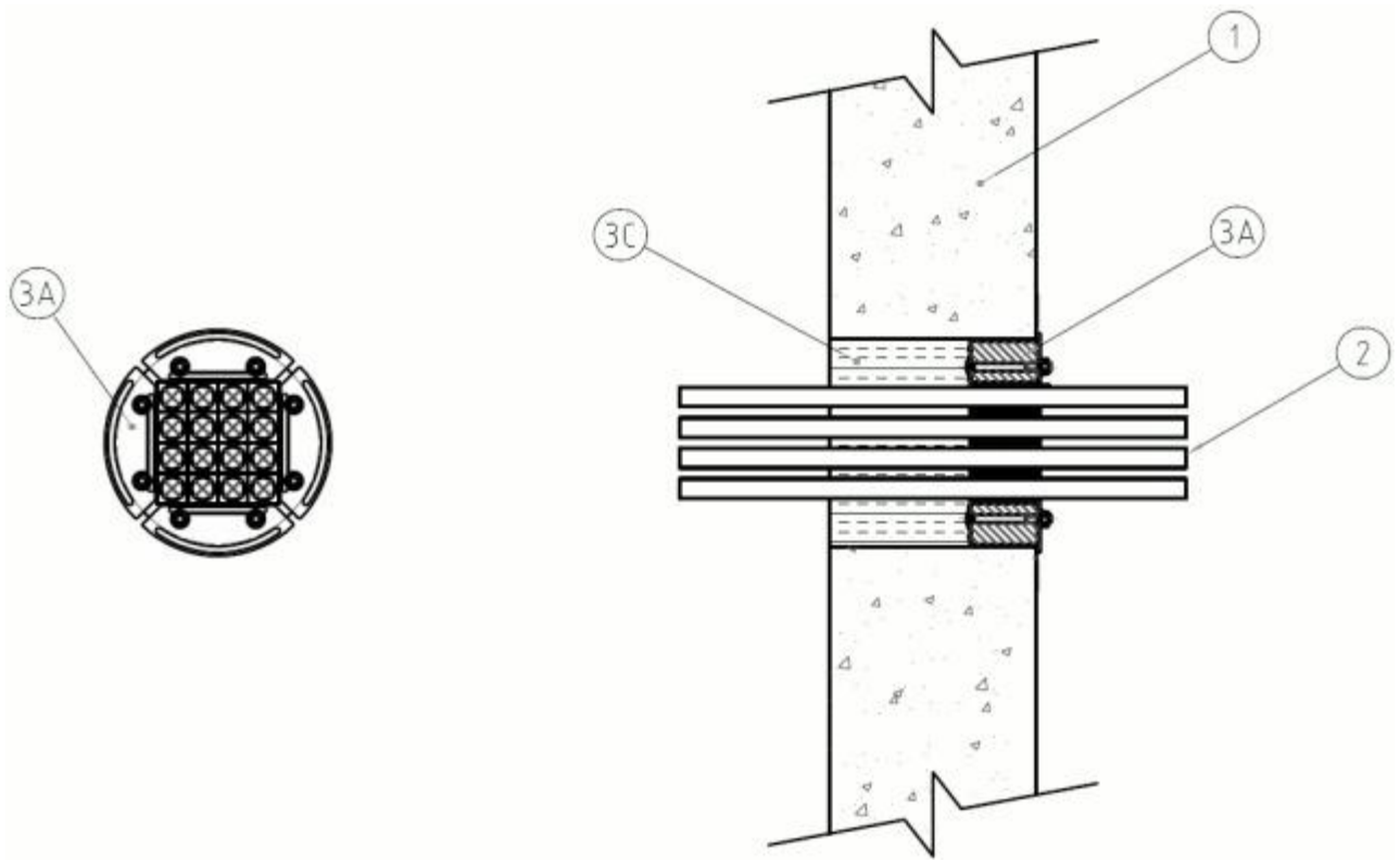
CONFIGURATION A
